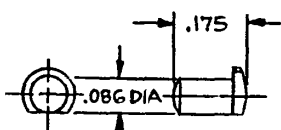
BUTTON MJ-102-G
